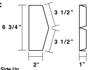
Ridge Cap* U-RC
