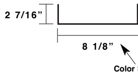
Jamb / Head Cover Trim ITHJ
