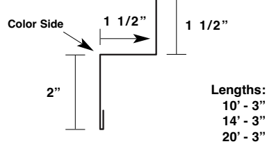
Outside Angle Trim ITOA
