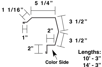
High Side Eave Trim* U-HS
