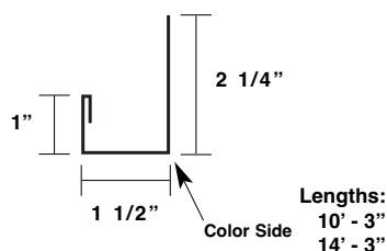
Sculptured Eave Trim* ITSCE
