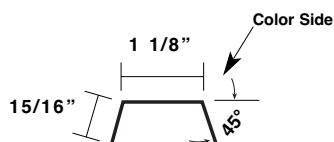
Gutter Strap U-GS
