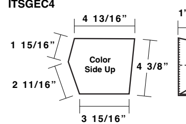
Standard Gutter End Cap 2:12 to 4:12 Pitch ITSGEC4
