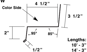
Inside Corner ITIC
