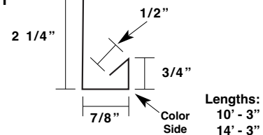
Sculptured Eave Trim* U-SE
