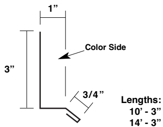
Masonry Wainscoat U-MW
