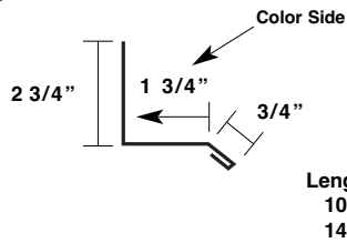
Masonry Wainscoat ITMW
