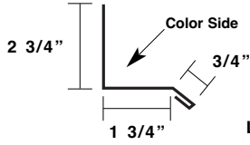
Simple Base Trim ITBD
