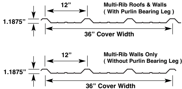
Multi-Rib
