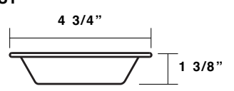
Aluminum Downspout Outlet BBPOUT
