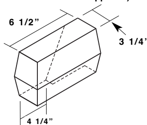
Gutter Corner Box For Standard Gutter 2:12 to 4:12 or with Sculptured Gutter (Right Hand Shown Left Hand Opposite) ITGCB
