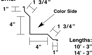
Inside Corner ITIC
