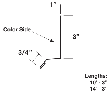
Outside Angle Trim
