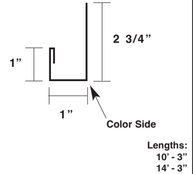
Inside Angle Trim
