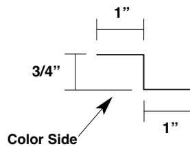
Zee Closure MT-184
