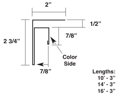
Zee Closure MT-184
