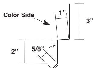
**Vertical Splice Trim
