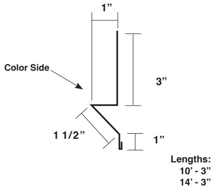
F and J x 1/2" MTFJ12
