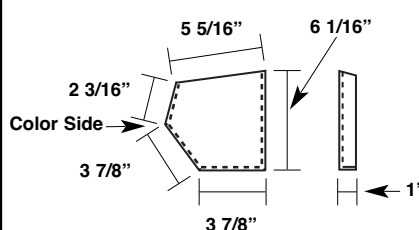
Gutter End Cap (2:12 to 4:12 Pitch) MLGE4
