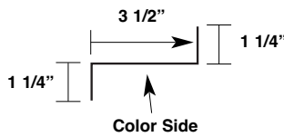
Insulation Zee Trim MLIZ
