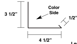
Commercial Rake Trim Item #: 38386
