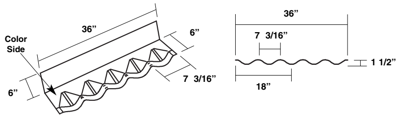
Contoured Hi-Side Tie-In Trim Item #: 38396
