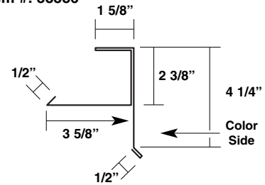
Commercial Rake Trim Item #: 38386
