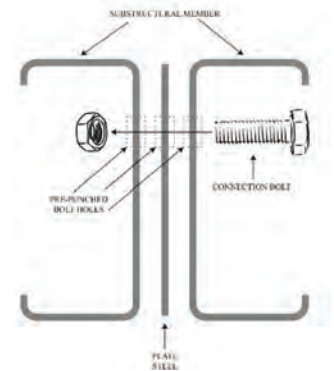
Example of Cold-Form Building Frame Construction
